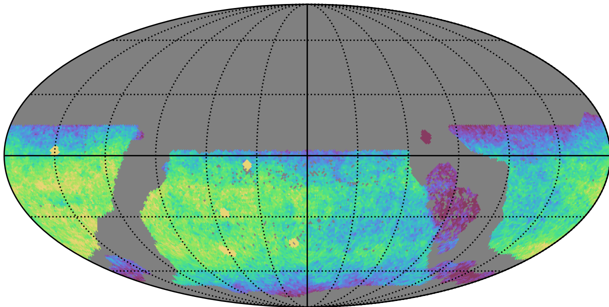
ddf_acor_sf25_lsf30_lsr50_v3.4_10yrs WFD u band: CoaddM5
