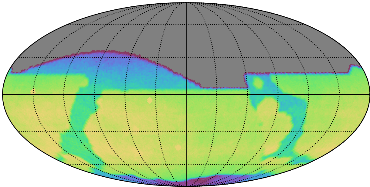
ddf_acor_sf25_lsf30_lsr50_v3.4_10yrs All sky r band: CoaddM5
