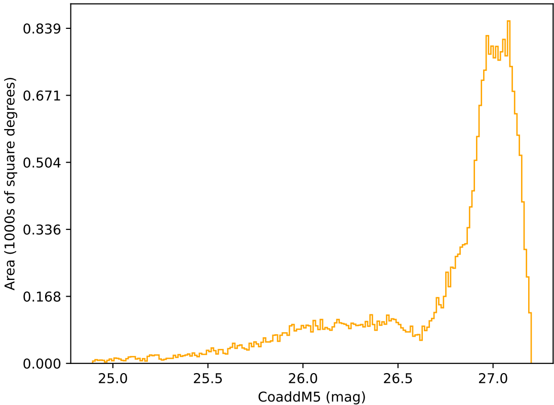
ddf_acor_sf25_lsf30_lsr50_v3.4_10yrs All sky r band: CoaddM5
