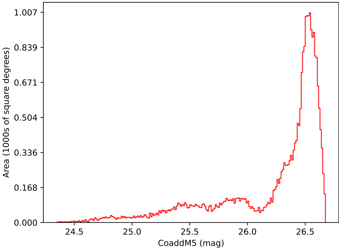
ddf_acor_sf25_lsf30_lsr50_v3.4_10yrs All sky i band: CoaddM5
