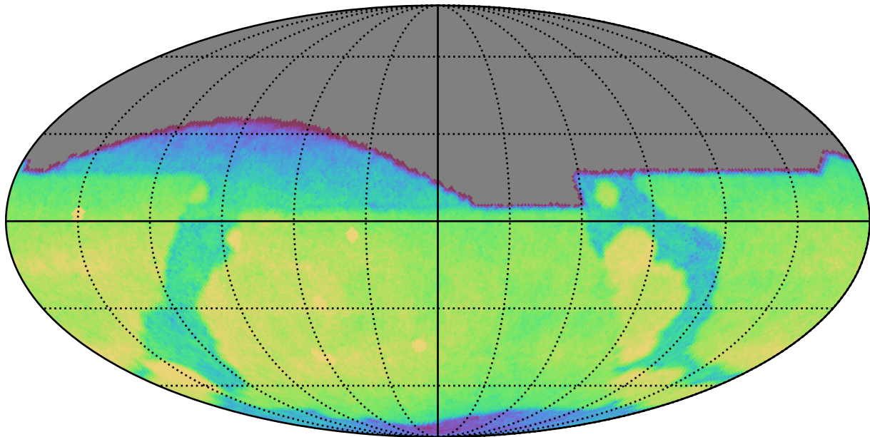
ddf_acor_sf25_lsf30_lsr50_v3.4_10yrs All sky g band: CoaddM5
