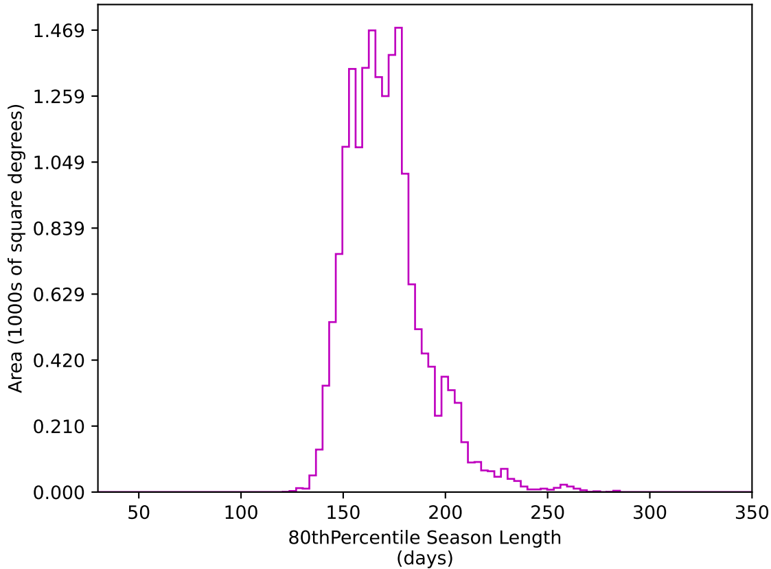
ddf_acor_sf25_lsf30_lsr50_v3.4_10yrs WFD z band: 80thPercentile Season Length
