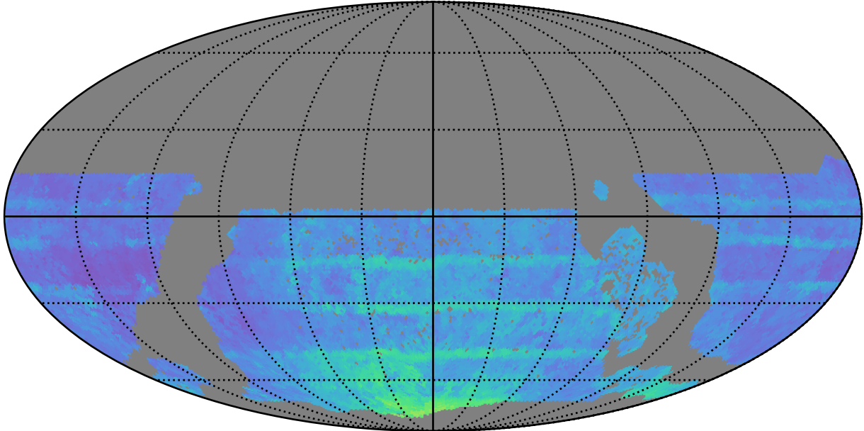
ddf_acor_sf25_lsf30_lsr50_v3.4_10yrs WFD all bands: 80thPercentile Season Length
