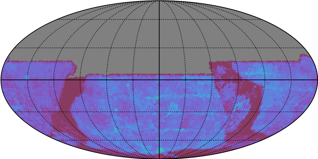
ddf_acor_sf25_lsf30_lsr50_v3.4_10yrs All sky u band: 80thPercentile Season Length
