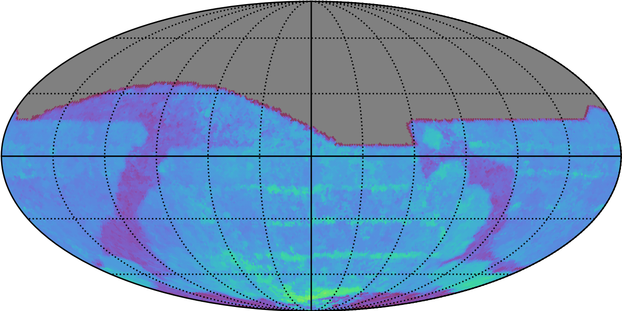
ddf_acor_sf25_lsf30_lsr50_v3.4_10yrs All sky i band: 80thPercentile Season Length
