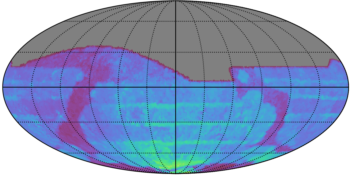
ddf_acor_sf25_lsf30_lsr50_v3.4_10yrs All sky all bands: 80thPercentile Season Length
