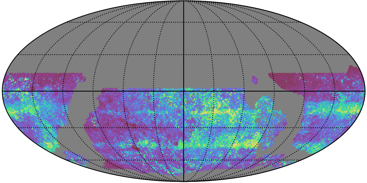
ddf_acor_sf25_lsf30_lsr50_v3.4_10yrs WFD zy bands: 75th Percentile Intranight Timespan
