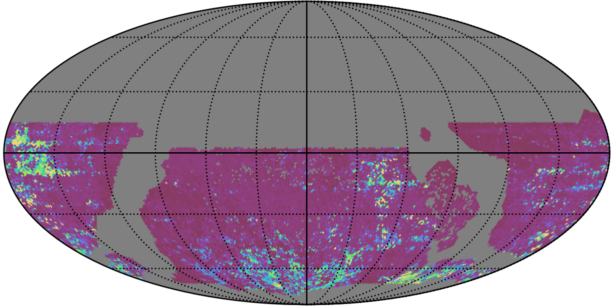
ddf_acor_sf25_lsf30_lsr50_v3.4_10yrs WFD z band: 75th Percentile Intranight Timespan
