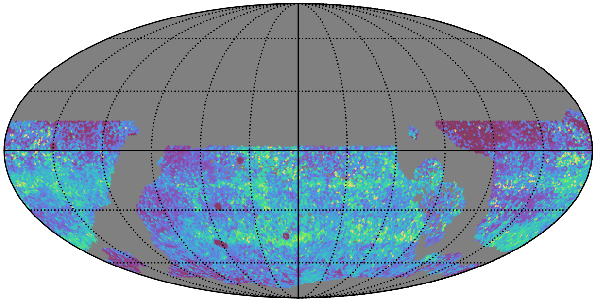
ddf_acor_sf25_lsf30_lsr50_v3.4_10yrs WFD y band: 75th Percentile Intranight Timespan
