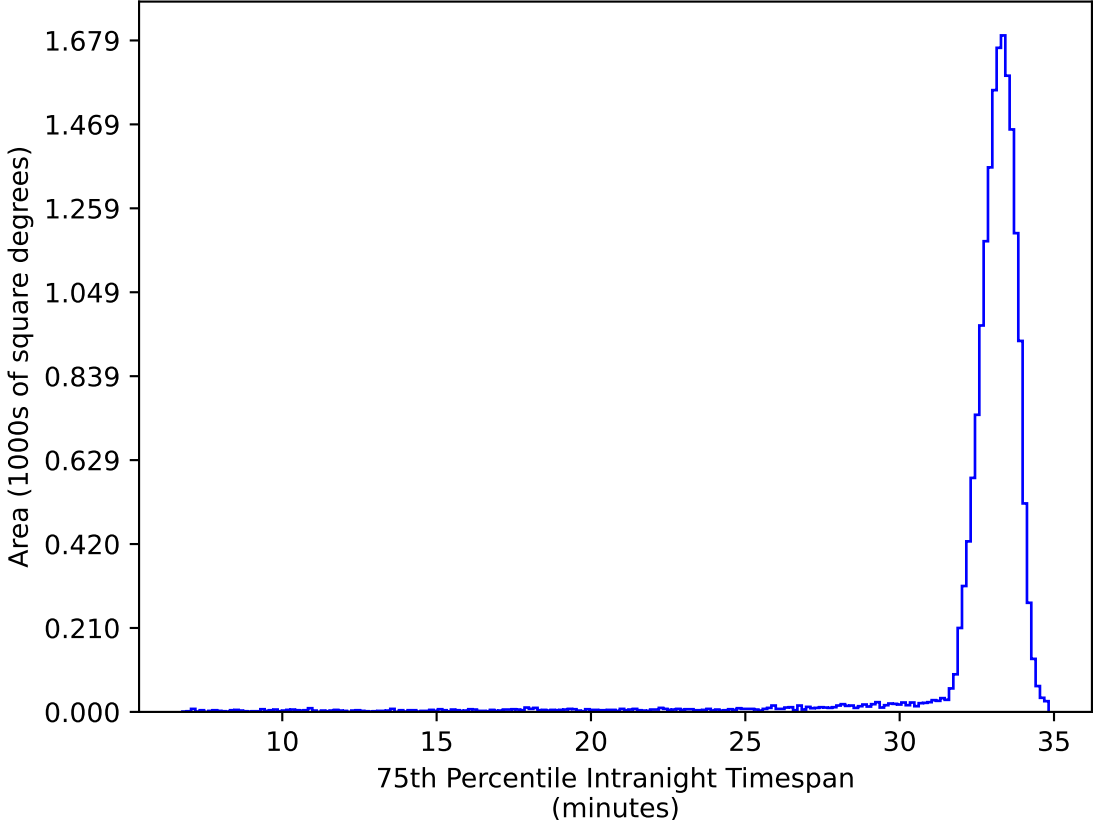
ddf_acor_sf25_lsf30_lsr50_v3.4_10yrs WFD ug bands: 75th Percentile Intranight Timespan
