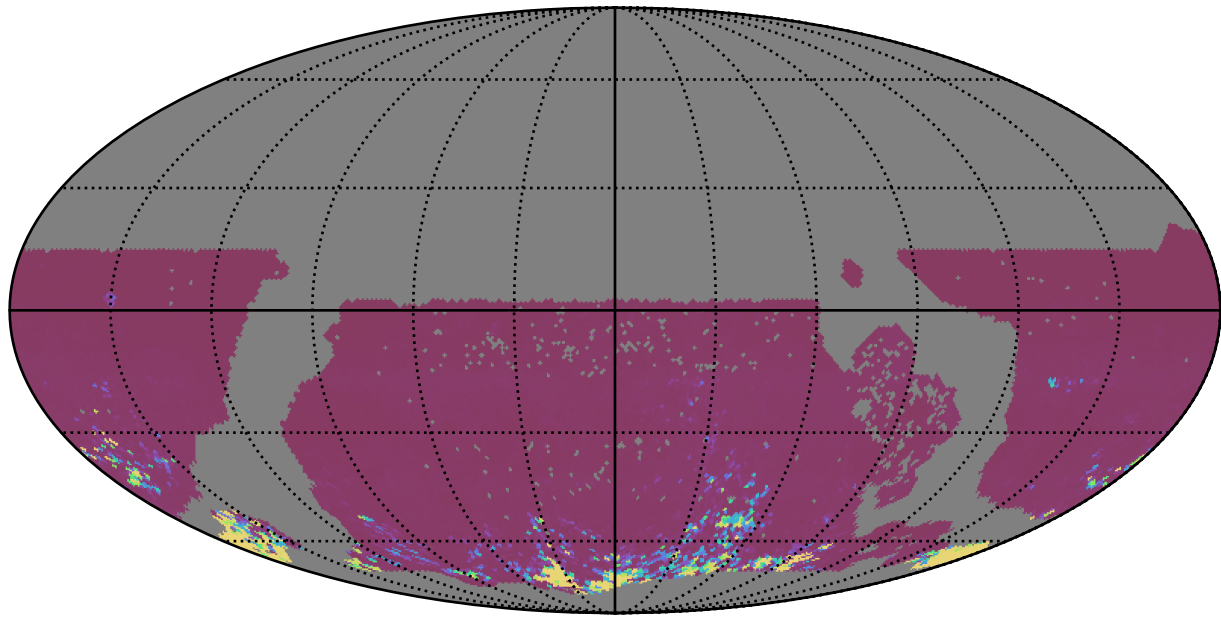
ddf_acor_sf25_lsf30_lsr50_v3.4_10yrs WFD ri bands: 75th Percentile Intranight Timespan
