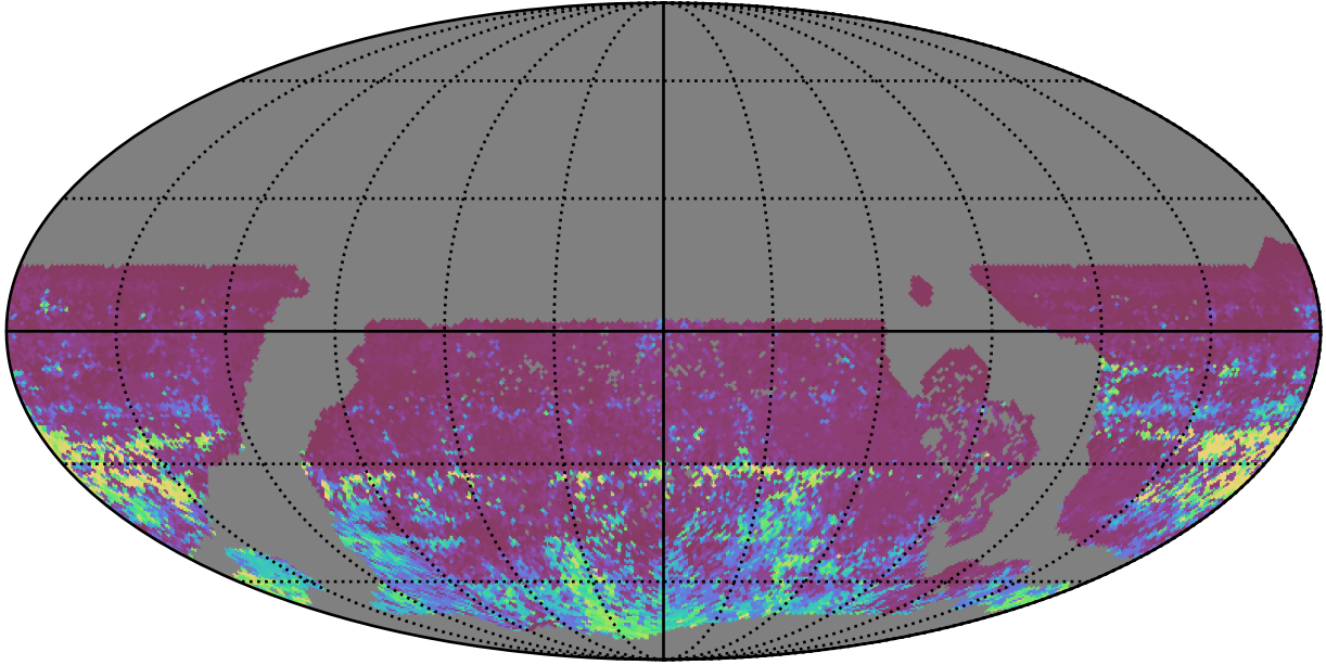
ddf_acor_sf25_lsf30_lsr50_v3.4_10yrs WFD r band: 75th Percentile Intranight Timespan
