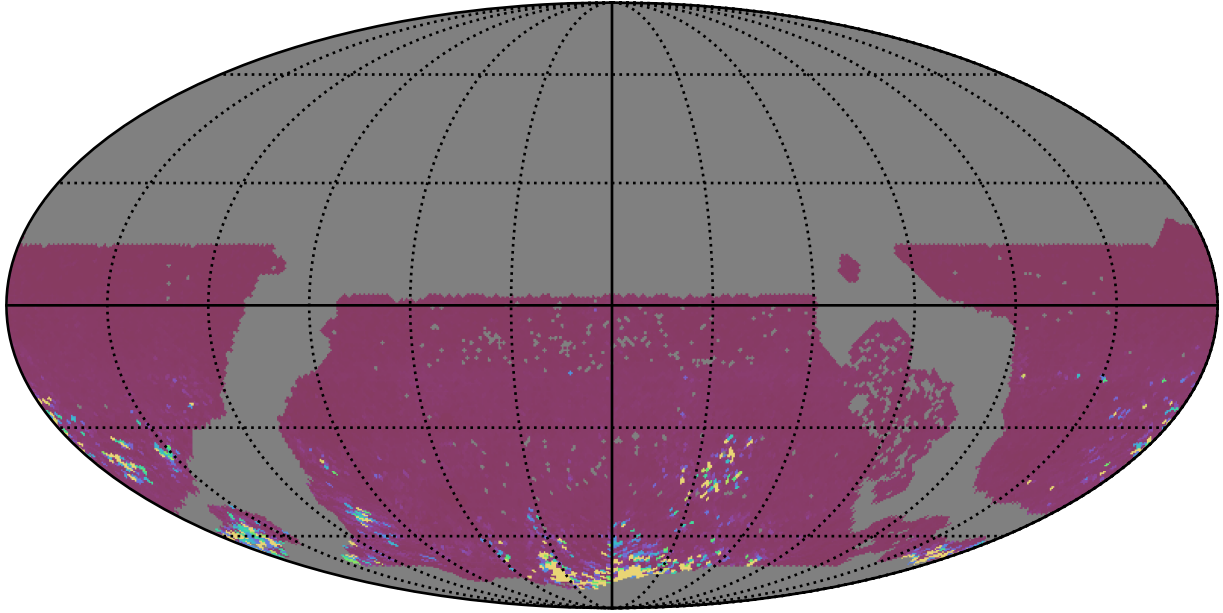
ddf_acor_sf25_lsf30_lsr50_v3.4_10yrs WFD gr bands: 75th Percentile Intranight Timespan
