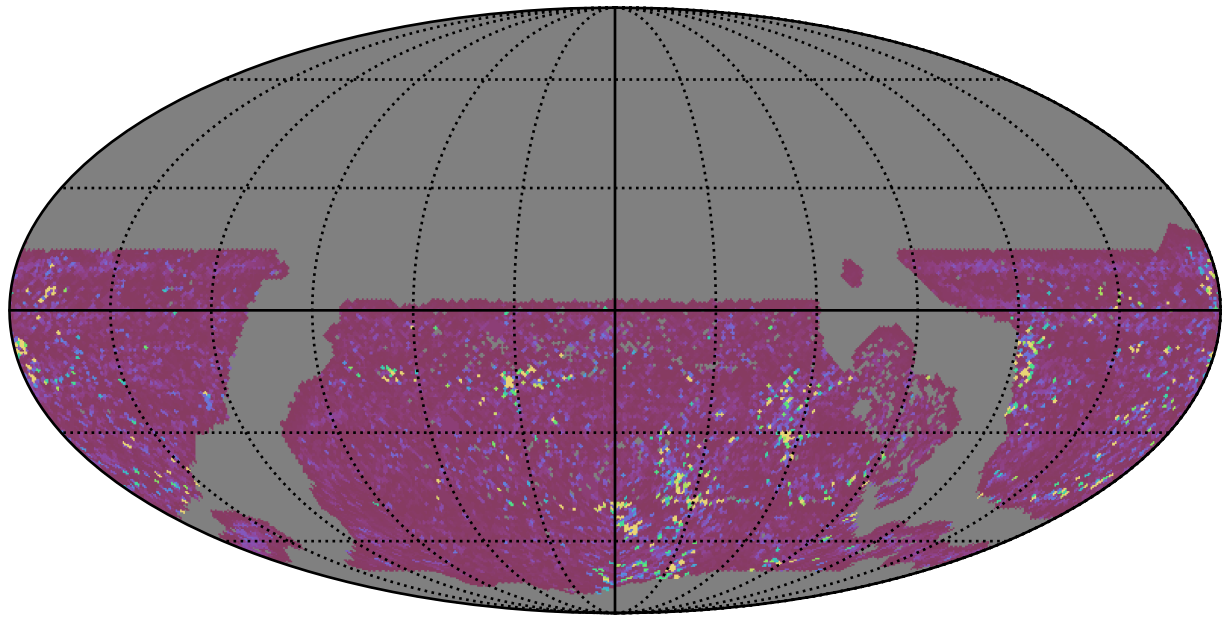
ddf_acor_sf25_lsf30_lsr50_v3.4_10yrs WFD g band: 75th Percentile Intranight Timespan
