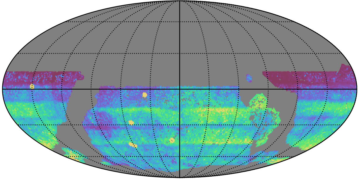
ddf_acor_sf25_lsf30_lsr50_v3.4_10yrs WFD all bands: 75th Percentile Intranight Timespan
