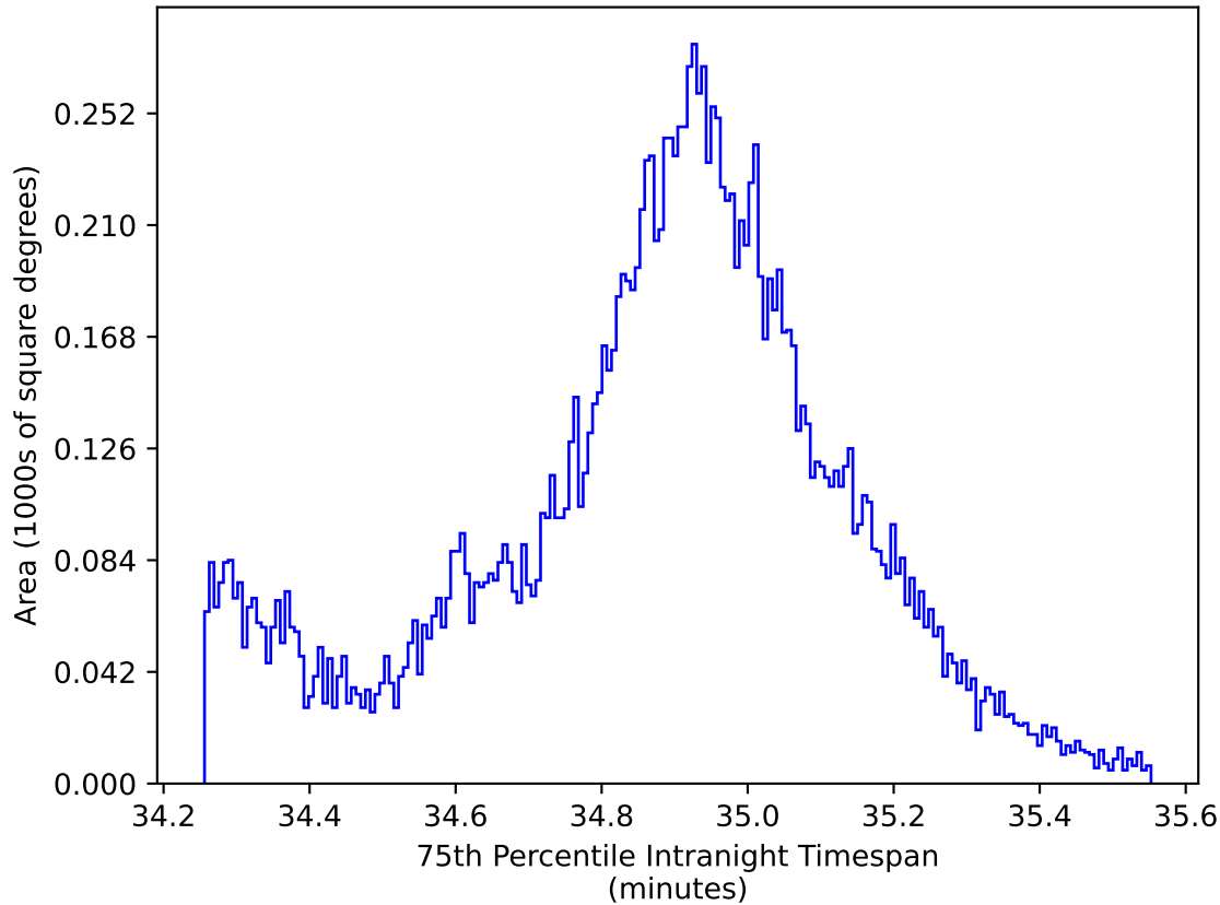
ddf_acor_sf25_ls30_lsr50_v3.4_10yrs WFD: 75th Percentile Intranight Timespan
