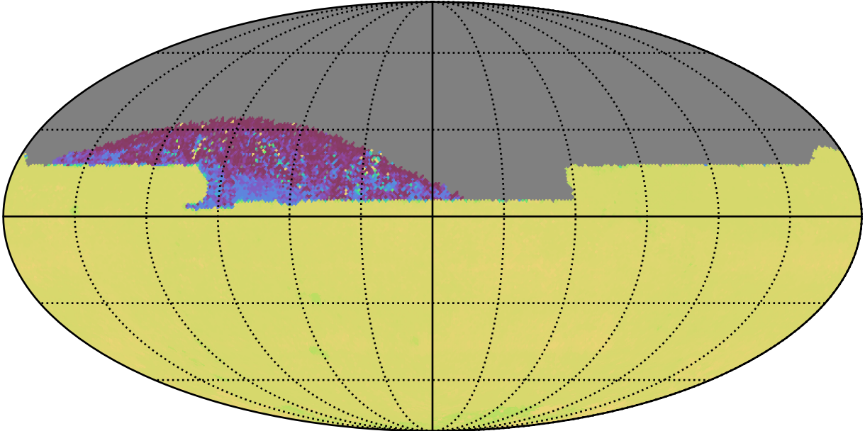
ddf_acor_sf25_lsf30_lsr50_v3.4_10yrs All sky zy bands: 75th Percentile Intranight Timespan
