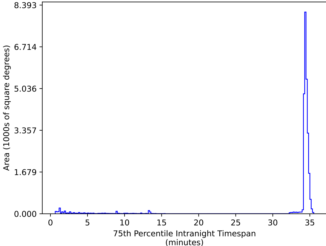
ddf_acor_sf25_lsf30_lsr50_v3.4_10yrs All sky zy bands: 75th Percentile Intranight Timespan
