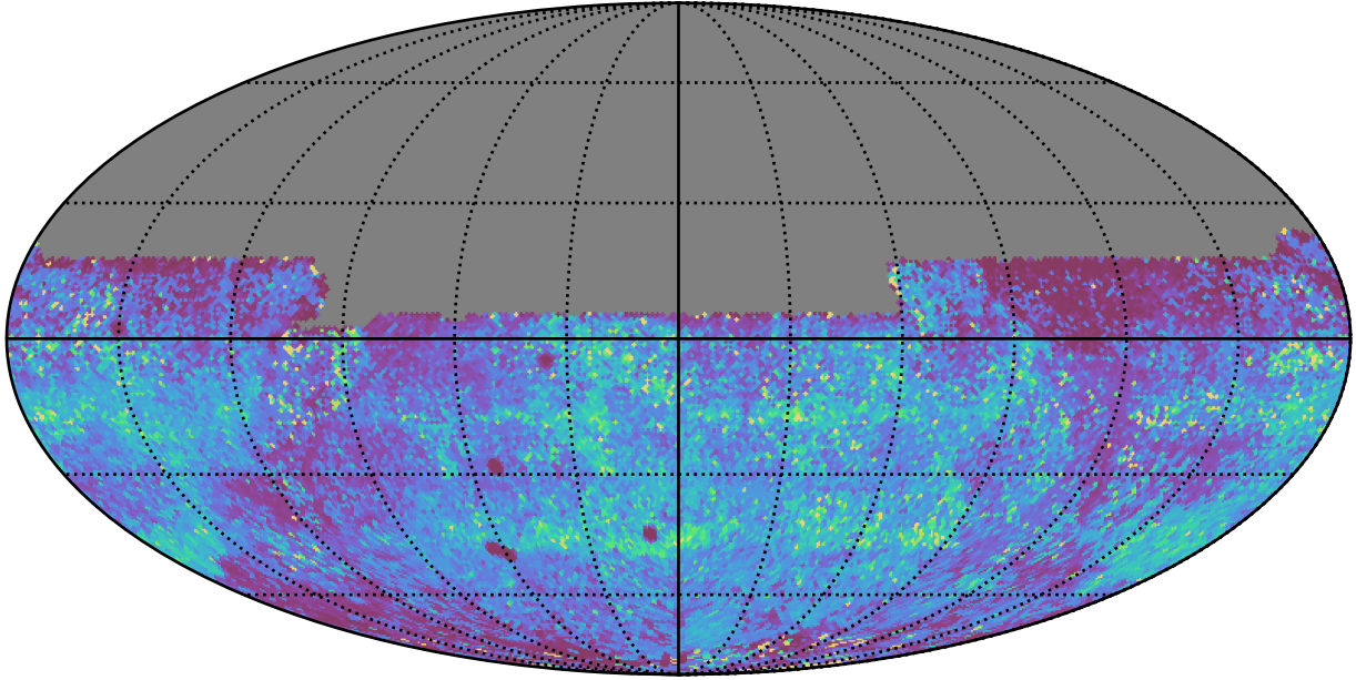
ddf_acor_sf25_lsf30_lsr50_v3.4_10yrs All sky y band: 75th Percentile Intranight Timespan
