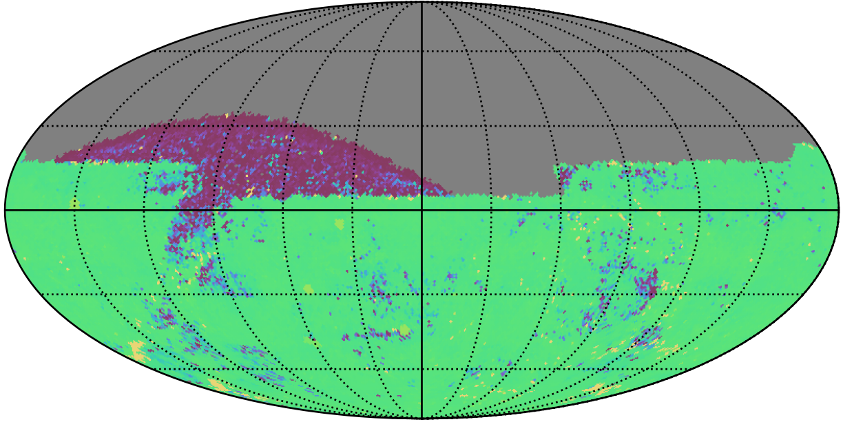
ddf_acor_sf25_lsf30_lsr50_v3.4_10yrs All sky ug bands: 75th Percentile Intranight Timespan
