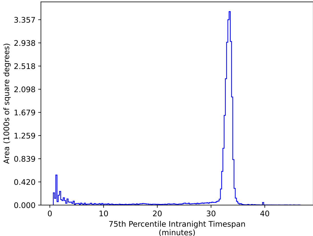
ddf_acor_sf25_lsf30_lsr50_v3.4_10yrs All sky ug bands: 75th Percentile Intranight Timespan
