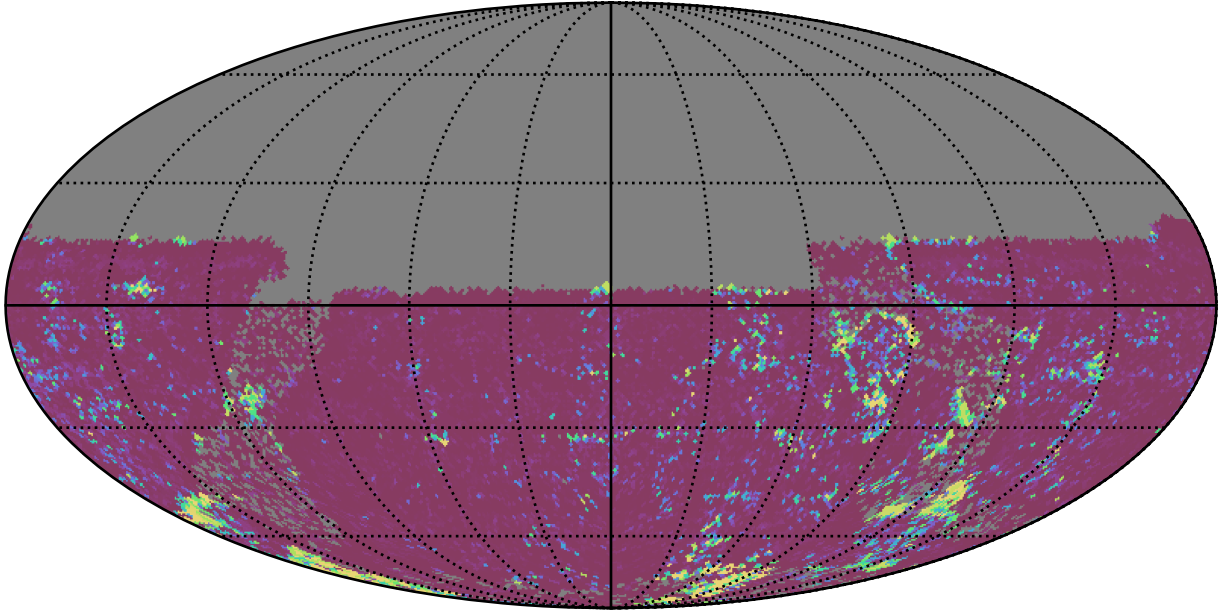
ddf_acor_sf25_lsf30_lsr50_v3.4_10yrs All sky u band: 75th Percentile Intranight Timespan
