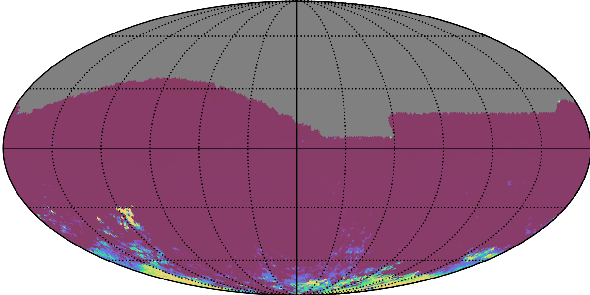
ddf_acor_sf25_lsf30_lsr50_v3.4_10yrs All sky ri bands: 75th Percentile Intranight Timespan
