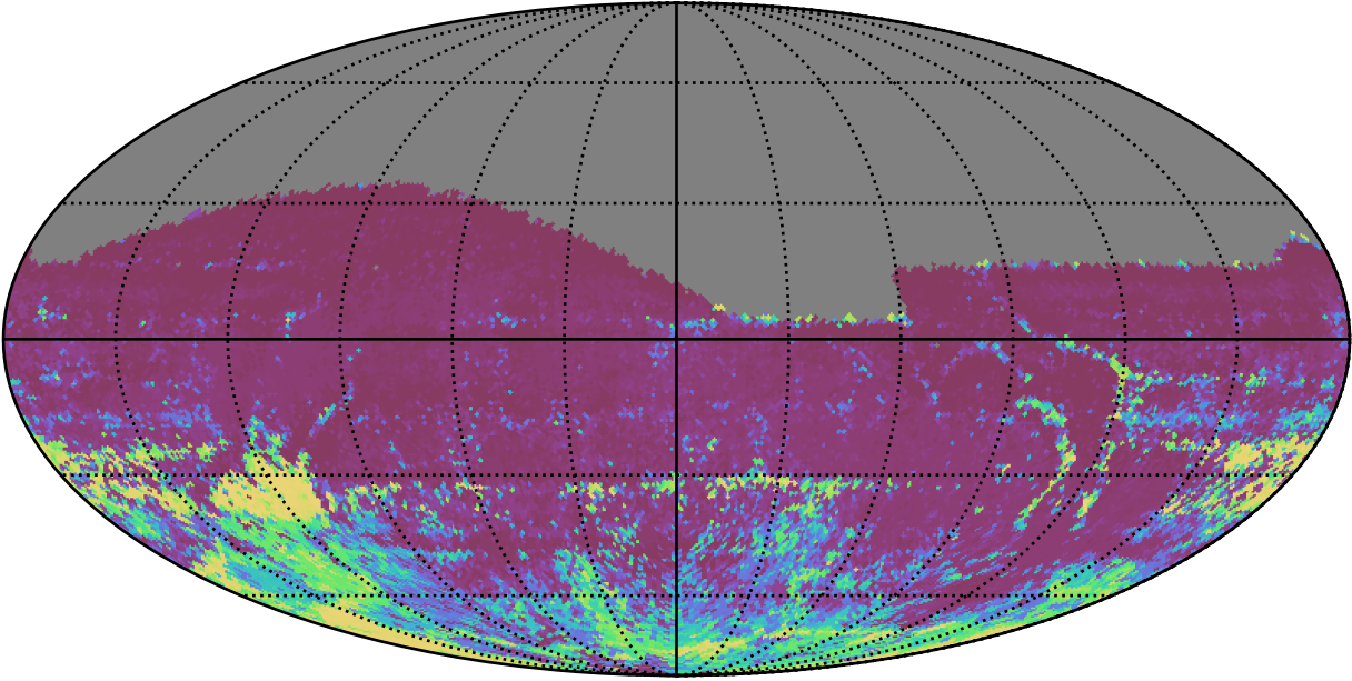
ddf_acor_sf25_lsf30_lsr50_v3.4_10yrs All sky r band: 75th Percentile Intranight Timespan
