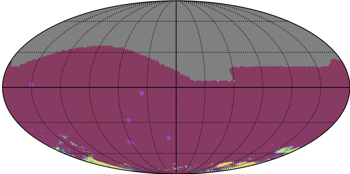
ddf_acor_sf25_lsf30_lsr50_v3.4_10yrs All sky iz bands: 75th Percentile Intranight Timespan
