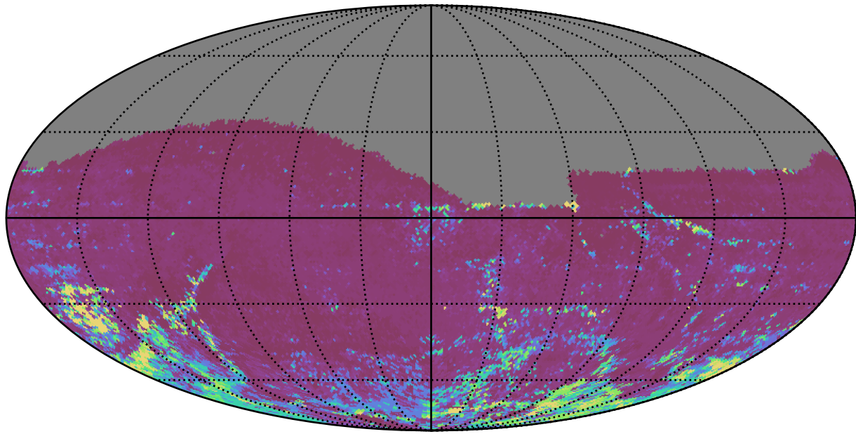
ddf_acor_sf25_lsf30_lsr50_v3.4_10yrs All sky i band: 75th Percentile Intranight Timespan
