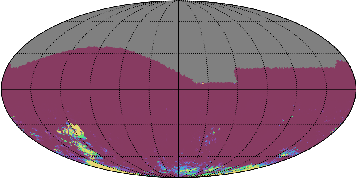
ddf_acor_sf25_lsf30_lsr50_v3.4_10yrs All sky gr bands: 75th Percentile Intranight Timespan
