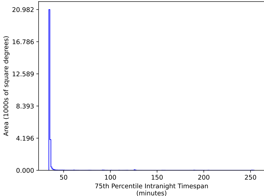
ddf_acor_sf25_lsf30_lsr50_v3.4_10yrs All sky gr bands: 75th Percentile Intranight Timespan
