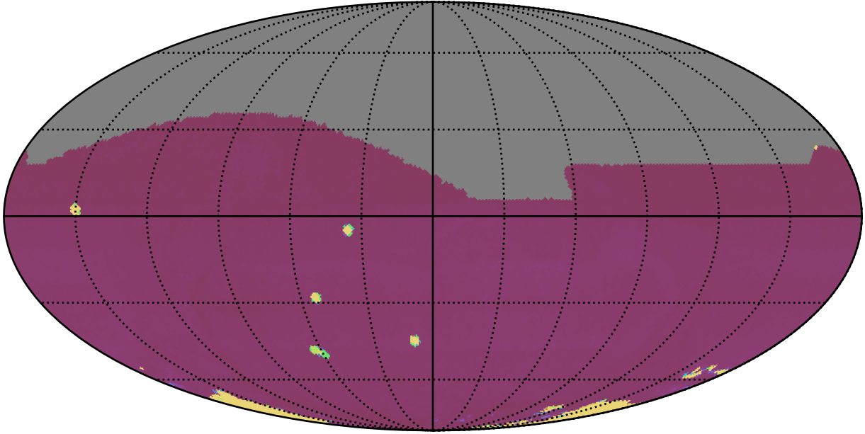
ddf_acor_sf25_lsf30_lsr50_v3.4_10yrs All sky all bands: 75th Percentile Intranight Timespan
