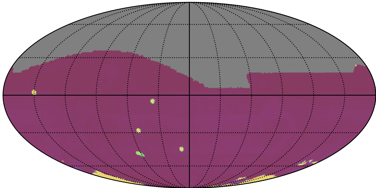
ddf_acor_sf25_lsf30_lsr50_v3.4_10yrs All sky: 75th Percentile Intranight Timespan
