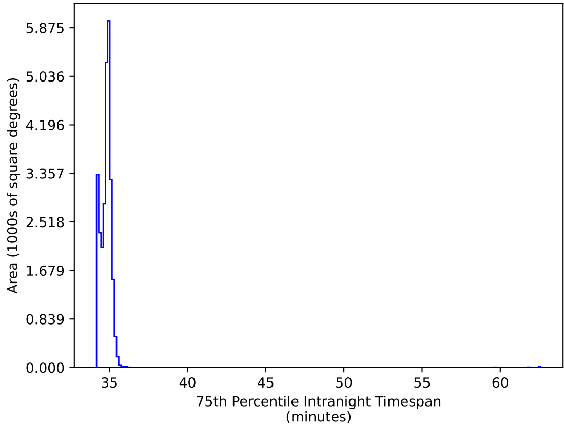
ddf_acor_sf25_lsf30_lsr50_v3.4_10yrs All sky: 75th Percentile Intranight Timespan
