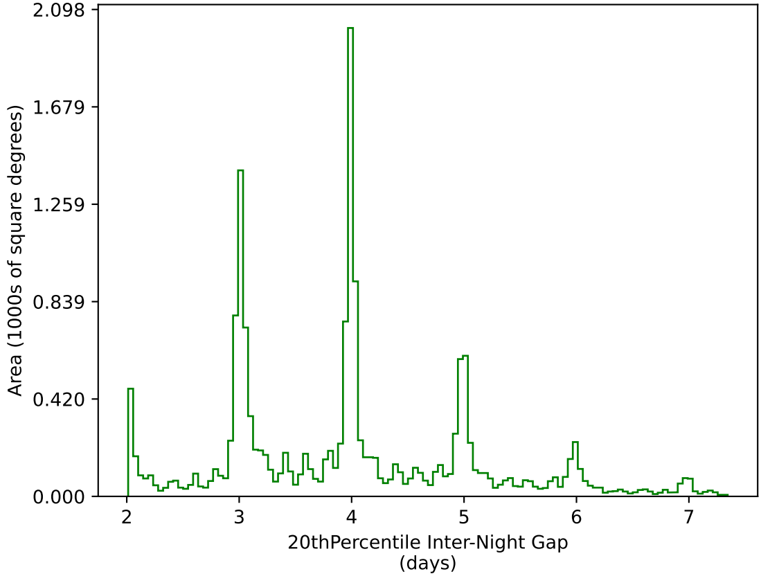
ddf_acor_sf25_lsf30_lsr50_v3.4_10yrs WFD g band: 20thPercentile Inter-Night Gap
