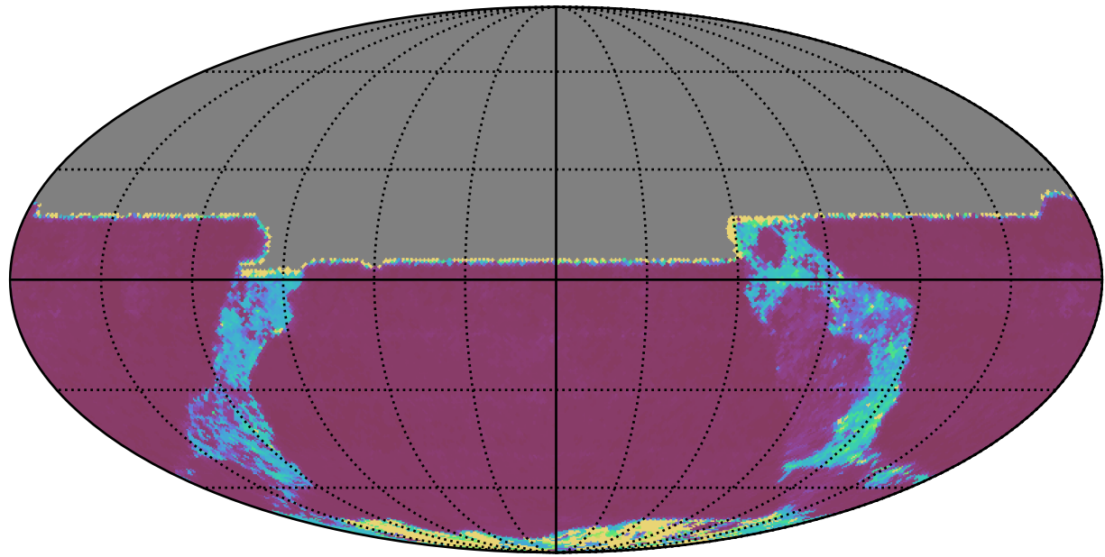
ddf_acor_sf25_lsf30_lsr50_v3.4_10yrs All sky y band: 20thPercentile Inter-Night Gap
