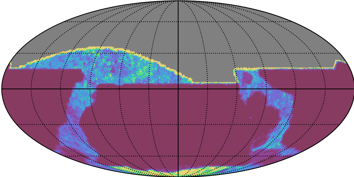
ddf_acor_sf25_lsf30_lsr50_v3.4_10yrs All sky all bands: 20thPercentile Inter-Night Gap
