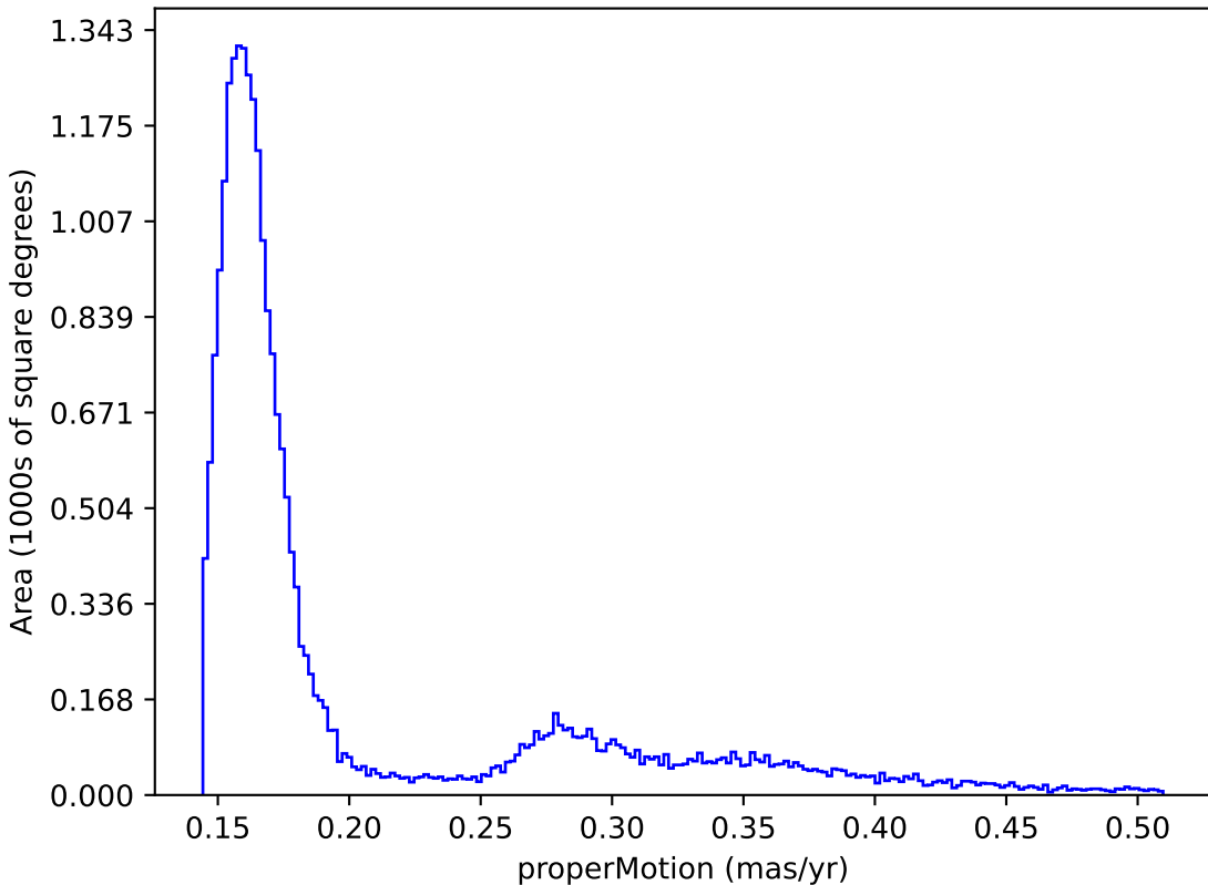
ddf_acor_sf25_lsf30_lsr50_v3.4_10yrs : properMotion
