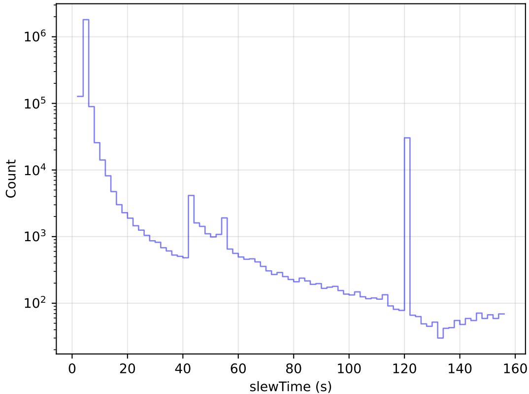
ddf_acor_sf25_lsf30_lsr50_v3.4_10yrs All visits: Slew Time Histogram
