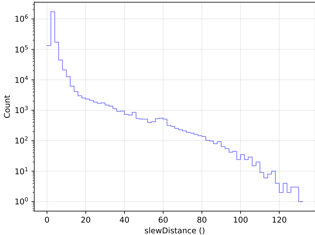
ddf_acor_sf25_lsf30_lsr50_v3.4_10yrs All visits: Slew Distance Histogram
