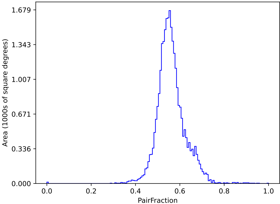
ddf_acor_sf25_lsf30_lsr50_v3.4_10yrs (g or r or i): PairFraction
