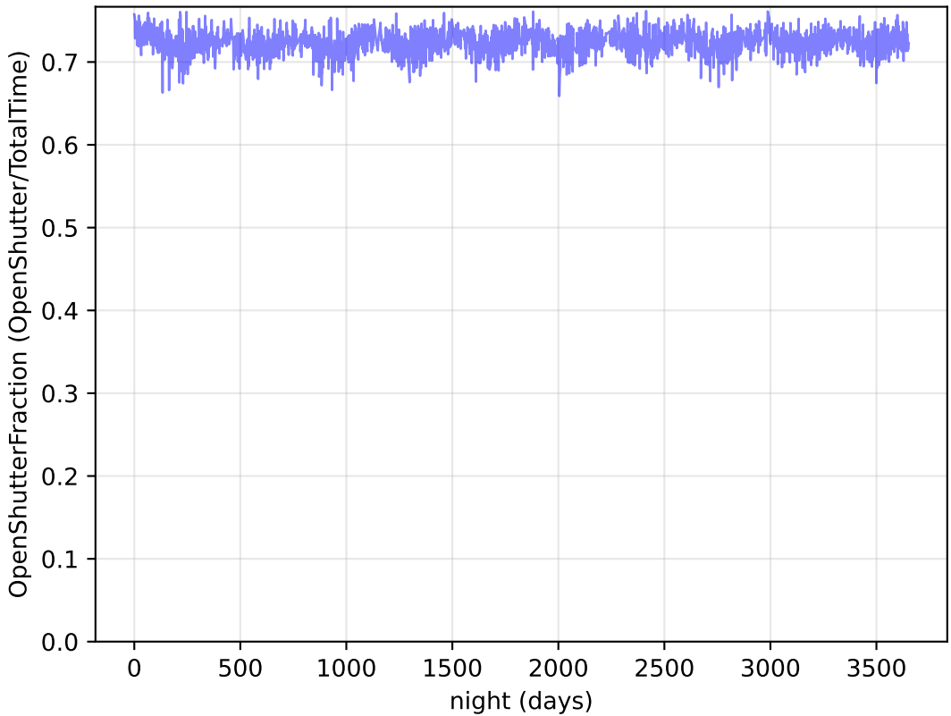
ddf_acor_sf25_lsf30_lsr50_v3.4_10yrs : OpenShutterFraction
