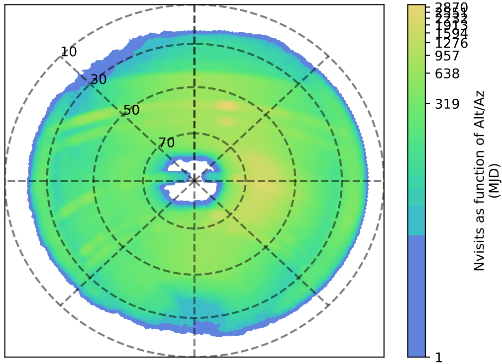
ddf_acor_sf25_lsf30_lsr50_v3.4_10yrs z: Nvisits as function of Alt/Az
