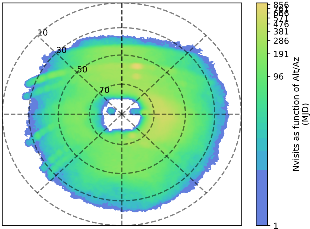
ddf_acor_sf25_lsf30_lsr50_v3.4_10yrs u: Nvisits as function of Alt/Az
