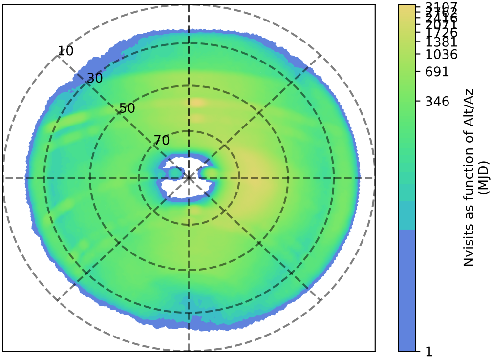
ddf_acor_sf25_lsf30_lsr50_v3.4_10yrs i: Nvisits as function of Alt/Az
