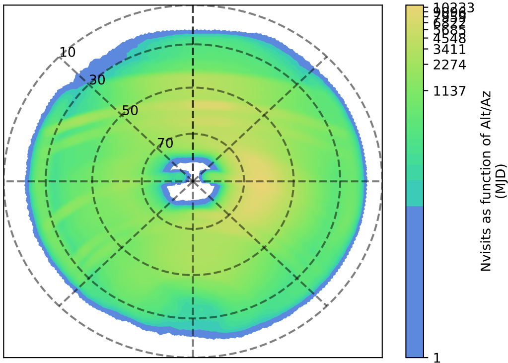
ddf_acor_sf25_lsf30_lsr50_v3.4_10yrs : Nvisits as function of Alt/Az
