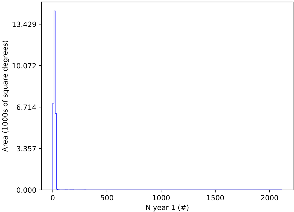
ddf_acor_sf25_lsf30_lsr50_v3.4_10yrs i and night < 365: N year 1
