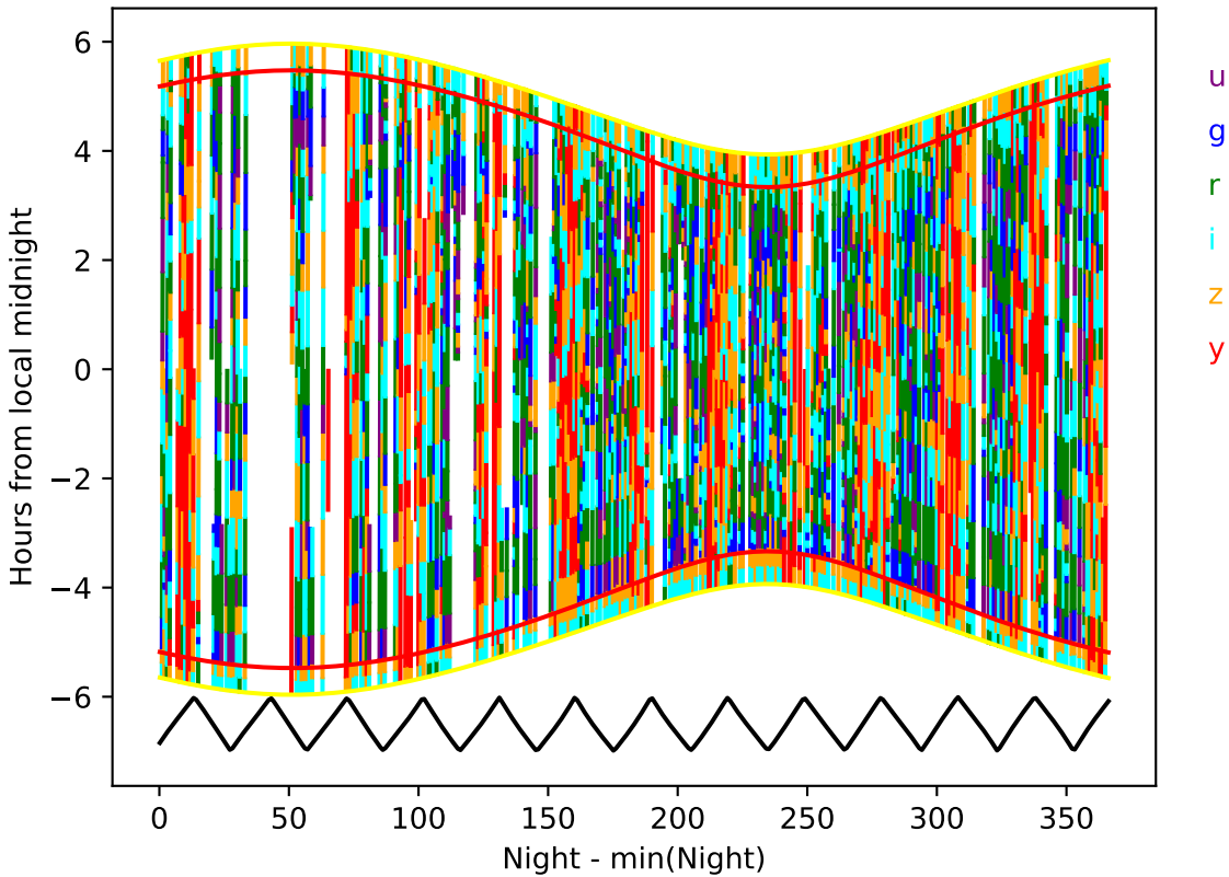
ddf_acor_sf25_lsf30_lsr50_v3.4_10yrs year 8-9: Hourglass
