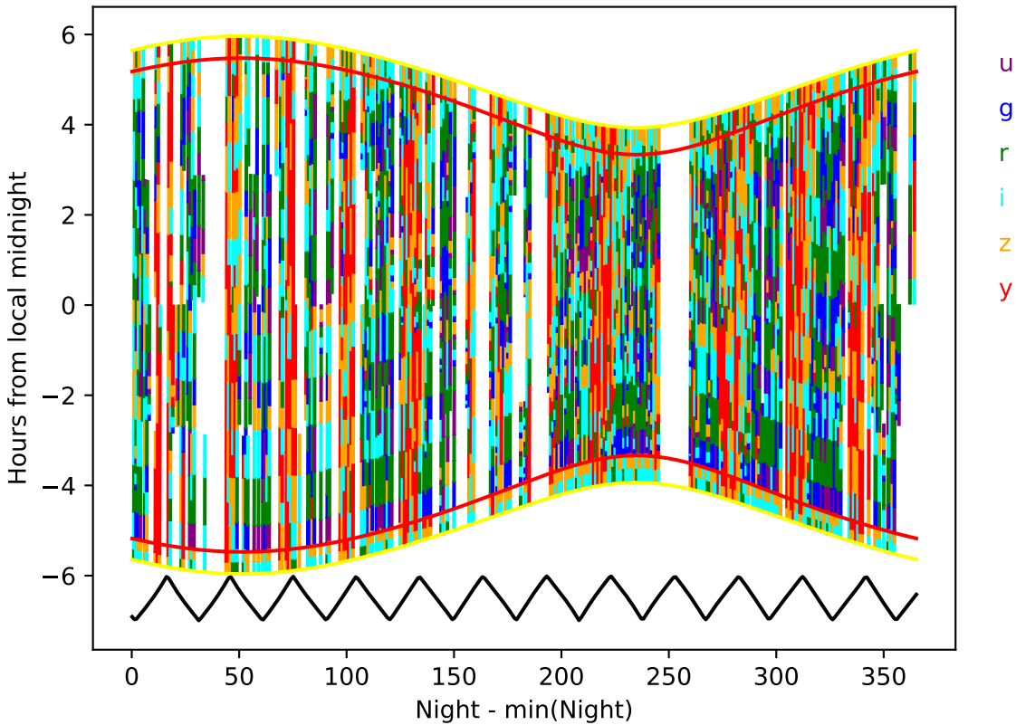
ddf_acor_sf25_lsf30_lsr50_v3.4_10yrs year 5-6: Hourglass
